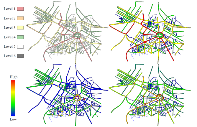
Fig. 3. Road significance measurement. Top: original road network containing six road levels (left) and significance value of road level (right); bottom: significance value of shape regularity (left) and combined significance value (right). The significance values are visualized by colors ranging from blue (lowest value) to red (highest value).
