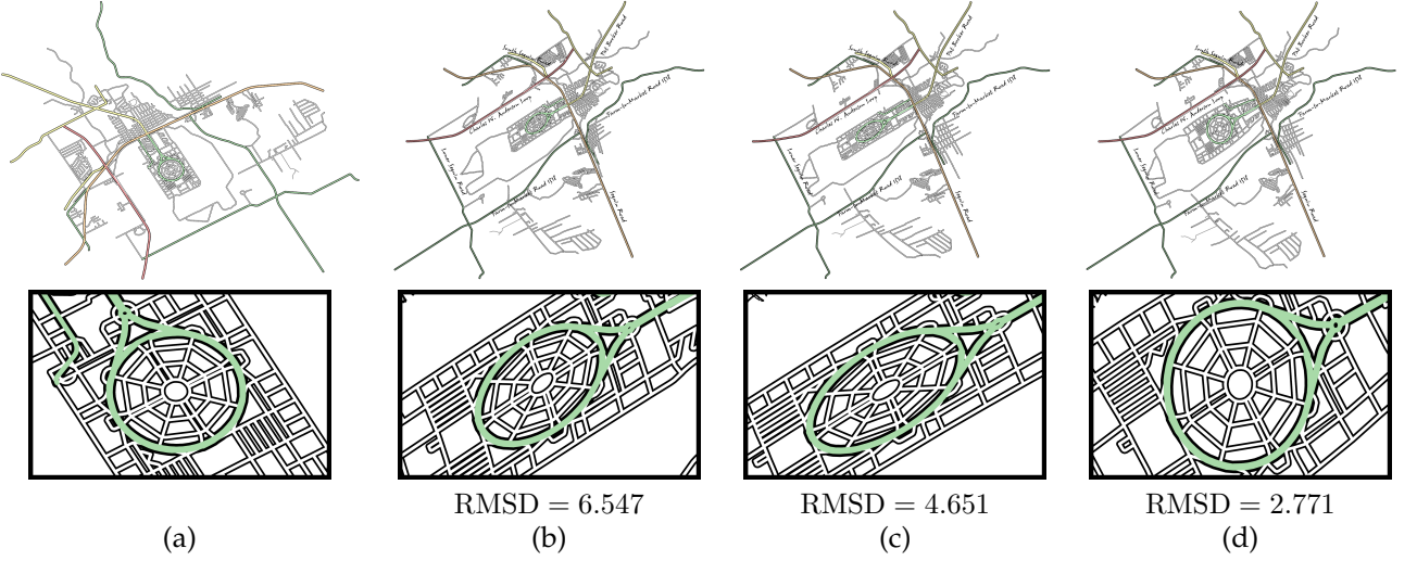
Fig. 16. Comparisons between our method, FBW [30] and TPS [31]. (a) Original road network; (b) result of FBW; (c) result of TPS; (d) our results. First row: original road network and warping results; second row: close-up views.
