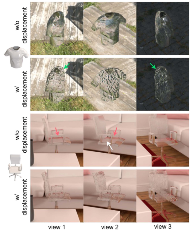
Fig. 13. Effect of anamorphic displacement optimization.
