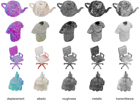
Fig. 9. Textured 3D model outputs produced by our method.
