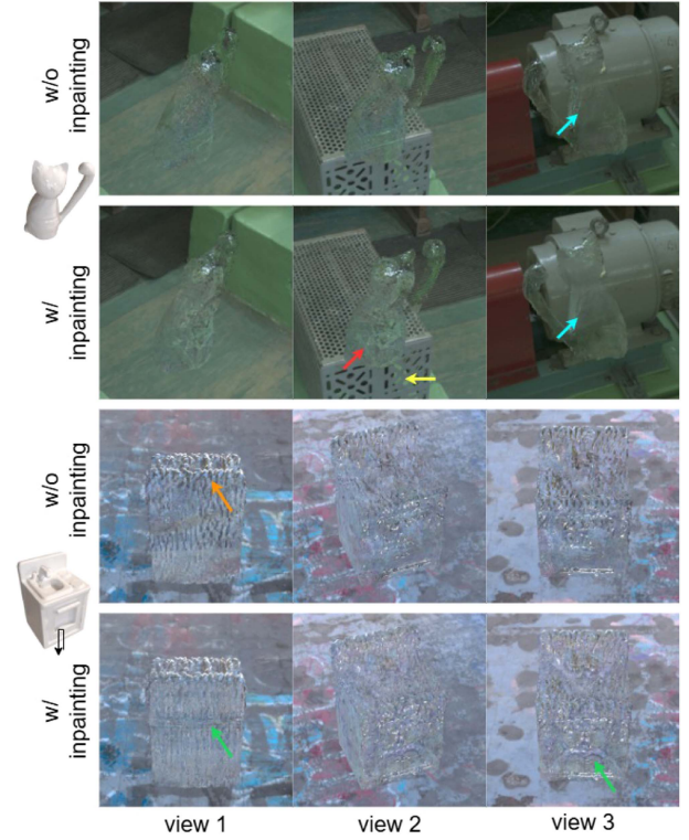
Fig. 14. Effect of using inpainting.
