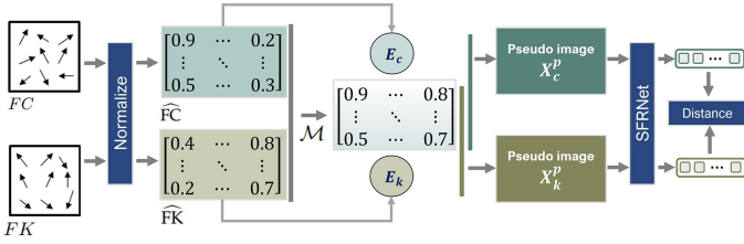
Fig. 4. Flowchart of our proposed PMSM.
