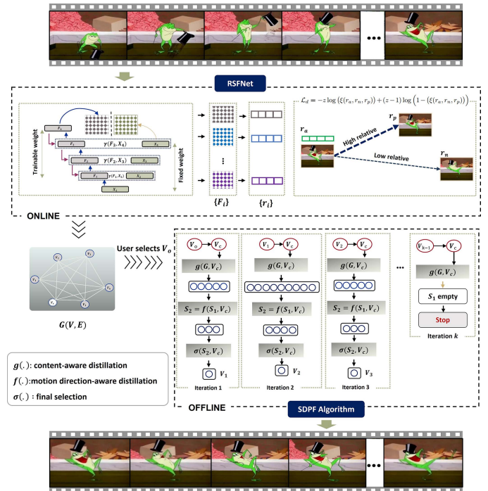
Fig. 1. Our framework for regenerating video sequence.
